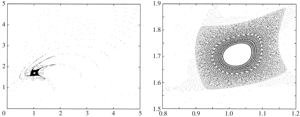
FIGURE 13. Poincaré section shown for \alpha^{(1\pm\epsilon)} = 5/2 , with an enlargement of the area close to the fixed point.
