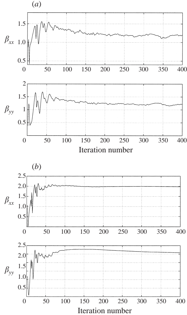
FIGURE 12. Horizontal and vertical dispersion for a blob above the core of the eddy for (a) \alpha^{(1\pm\epsilon)} = 3/5 and (b) \alpha^{(1\pm\epsilon)} = 6/5 (shown for 400 iterations). These are the same runs as shown in figure 11 but with additional white noise terms, corresponding to molecular diffusion. Note in comparison with the corresponding sub figures of figure 11 we unsurprisingly observe a slight increase in the level of diffusion.
