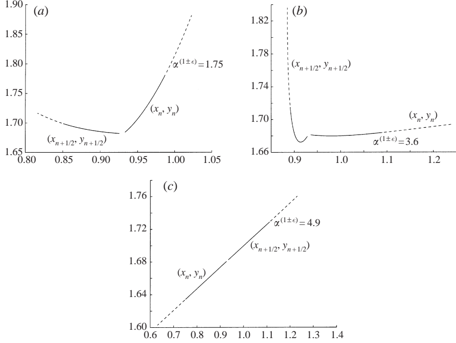
FIGURE 6. Bifurcation diagram for the fixed point of the maps. (a) Implicit in x , (b) implicit in y , (c) midpoint. The dotted line denotes where the modulus of the trace of the Jacobian at the fixed point exceeds 2, that is the Hessian becomes negative. The fixed points are shown for all three variations of the area-preserving map. We recall that these are fixed points of the map M , and not of R_1 and R_2 individually, hence we show (x_n, y_n) and R_1(x_n, y_n) . Notice that for small \alpha^{(1\pm\epsilon)} the fixed points are similar, but as this quantity increases they differ, and the central fixed points bifurcate at different values. The fixed points for the midpoint map compare well with Blake & Otto (1996) which exploits a continuous protocol.
